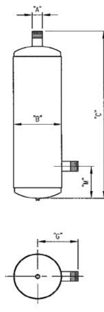
BEO-L Sizes 2 1/2" Thru 4"
