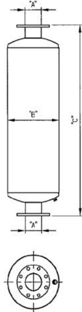
BEO Sizes 5" Thru 48"
