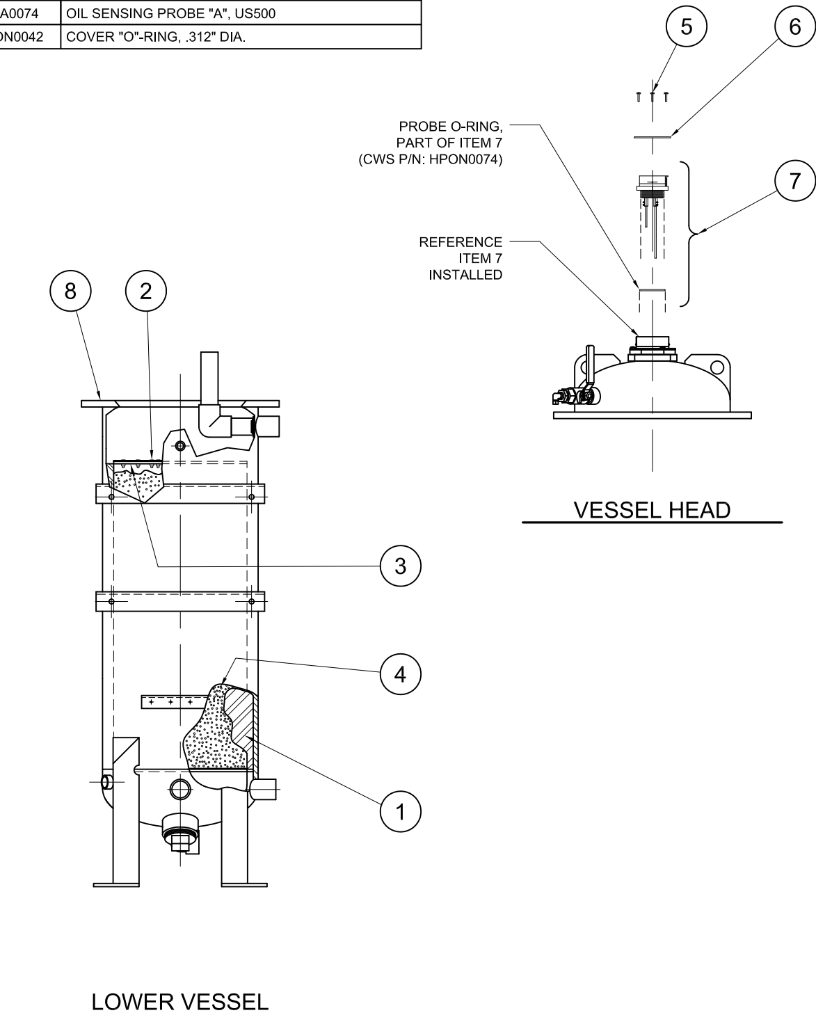
HELI-SEP 500 SUB-ASSEMBLY
