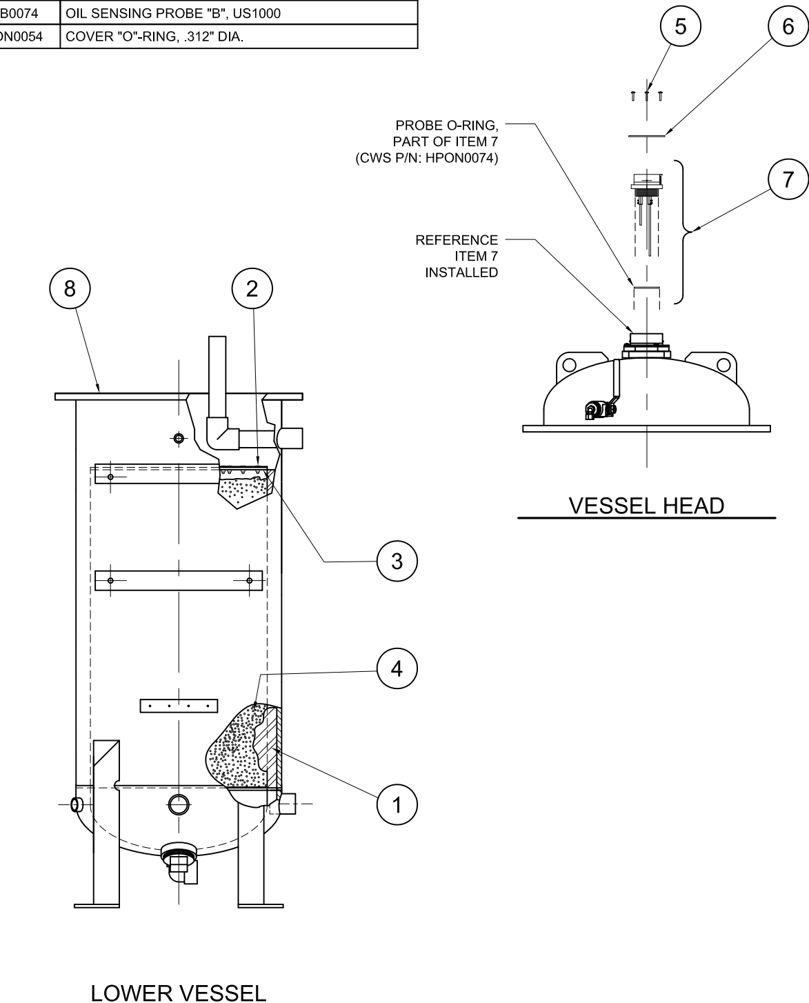
HELI-SEP 1000 SUB-ASSEMBLY
