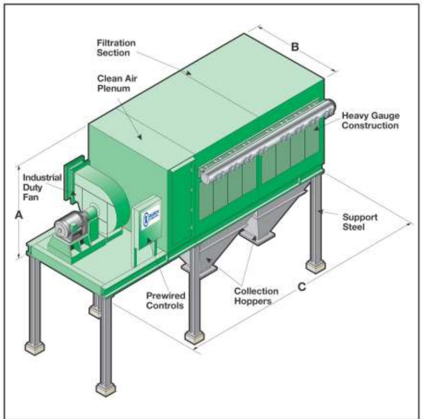
A typical WE Series unit arrangement.
