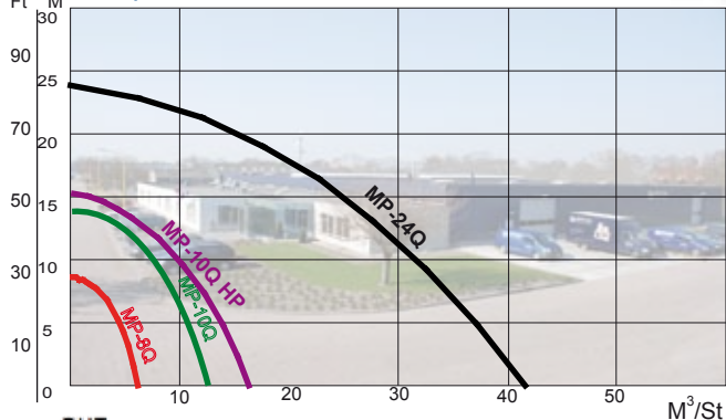
Pump Characteristics
