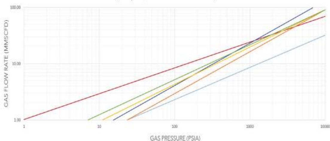
Flow Curve (at 2psid, at 0.65 SG and 68F)
