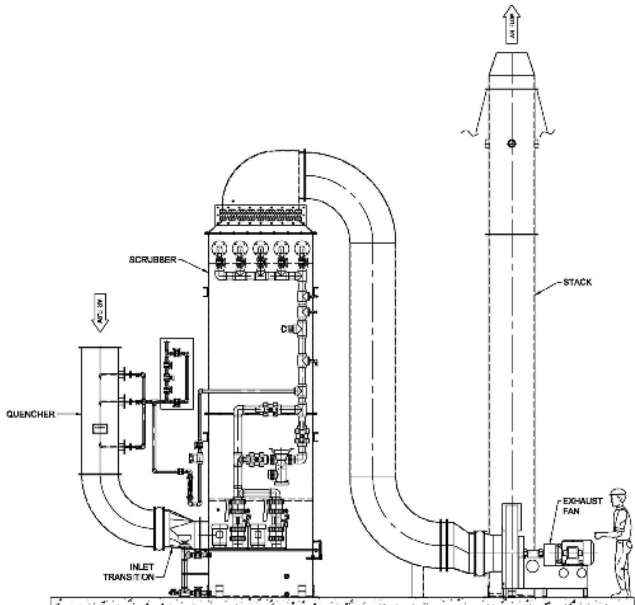
QUENCHER AND COUNTER CURRENT VERTICAL SCRUBBER SYSTEM
